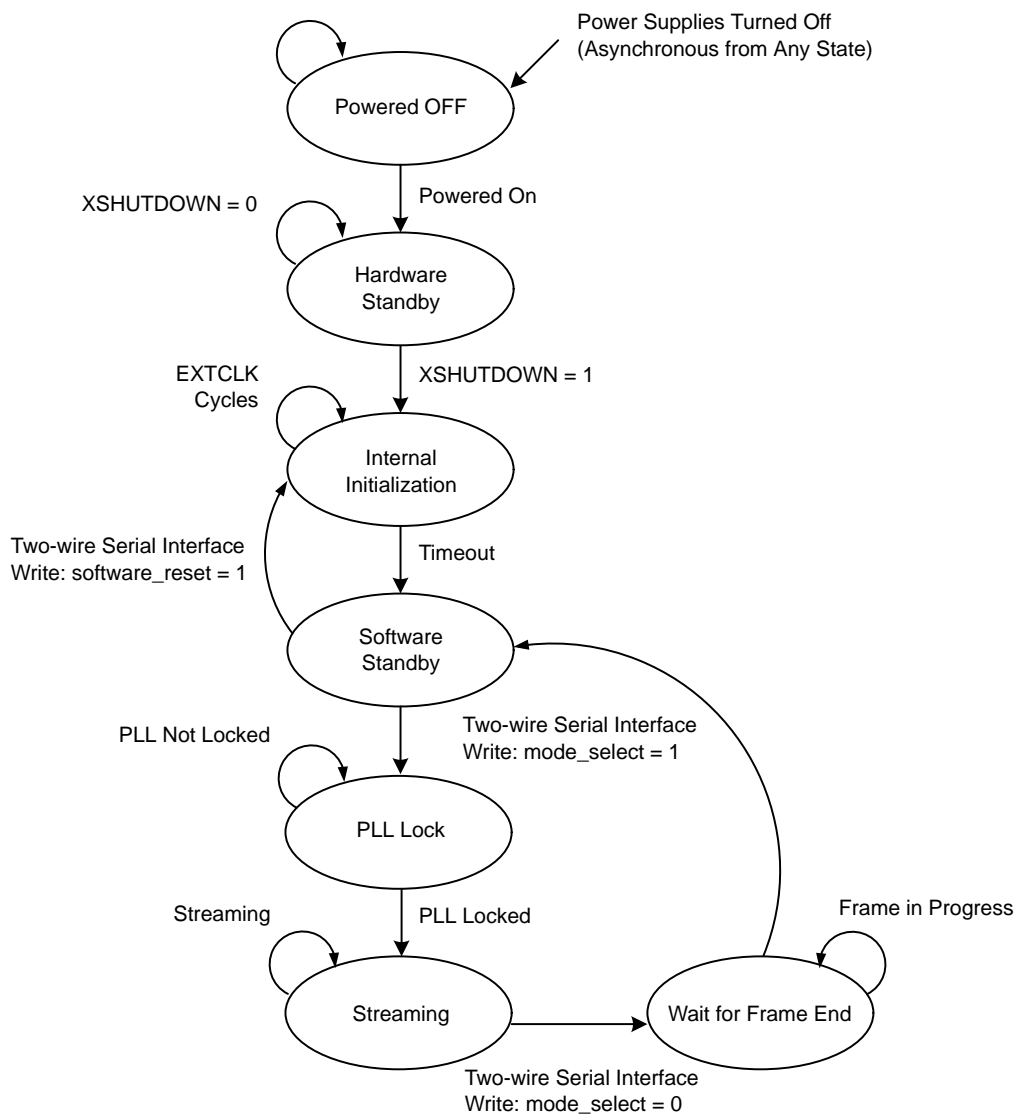
Figure 5. System States
