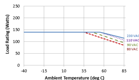
Convection – 48V to 56V Models
