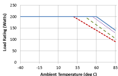
14 CFM Airflow – 12V to 19V Models
