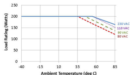
14 CFM Airflow – 48V to 56V Models
