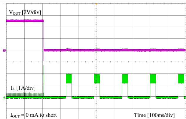
Figure 9-8. Short Protection
