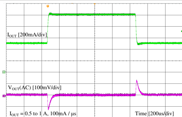
Figure 9-7. Load Transient
