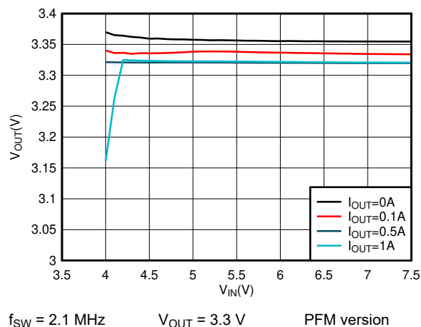
Figure 7-6. 3.3-V Dropout
