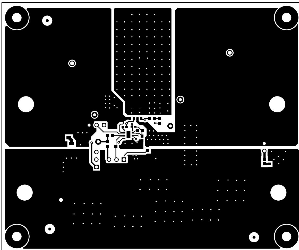
Figure 6-3. TOP Layer Routing
