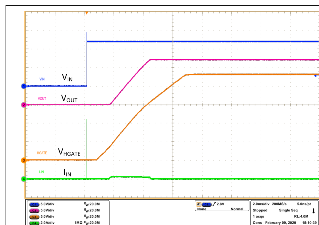
Figure 5-8. Hot-plug 12 V
