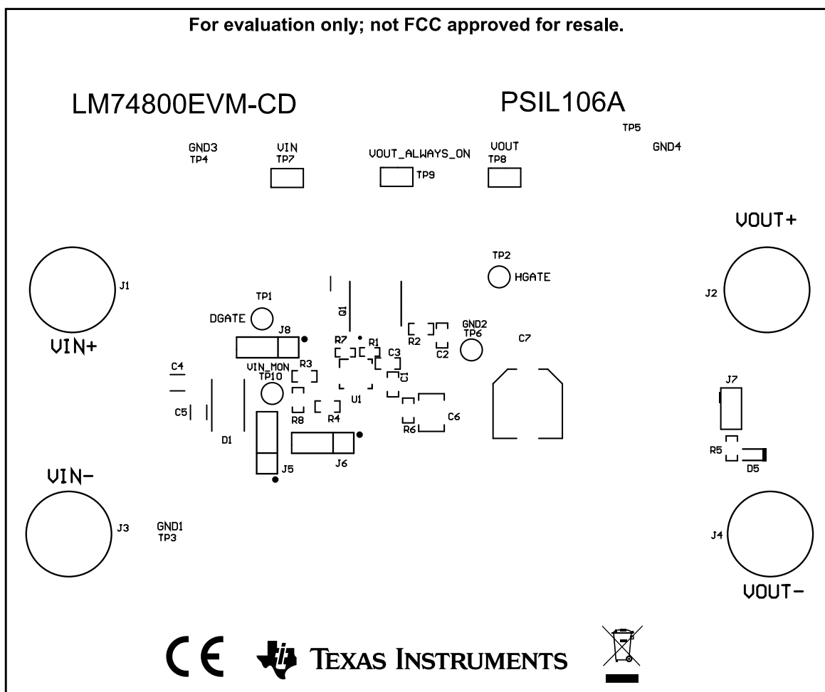
Figure 6-1. Component Placement TOP
