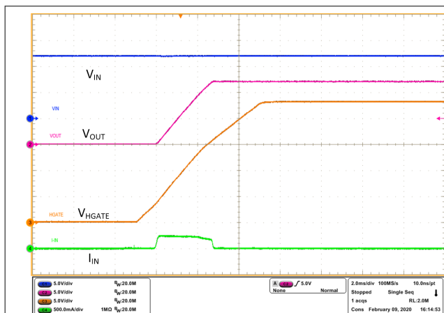
Figure 5-10. Inrush current with No Load
