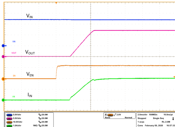
Figure 5-11. Inrush current with 6-Ω Load
