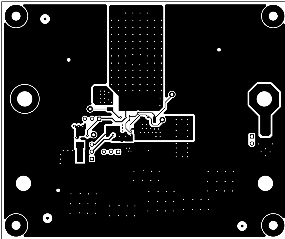
Figure 6-4. BOTTOM Layer Routing
