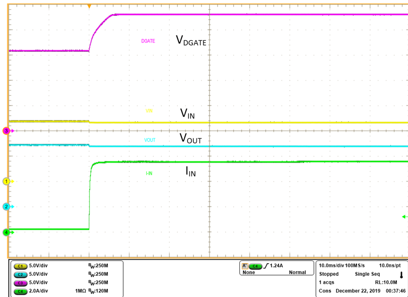
Figure 5-12. Load Transient Response 100 mA to 5 A
