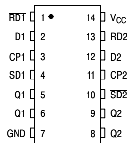
Figure 1. Pin Assignment
