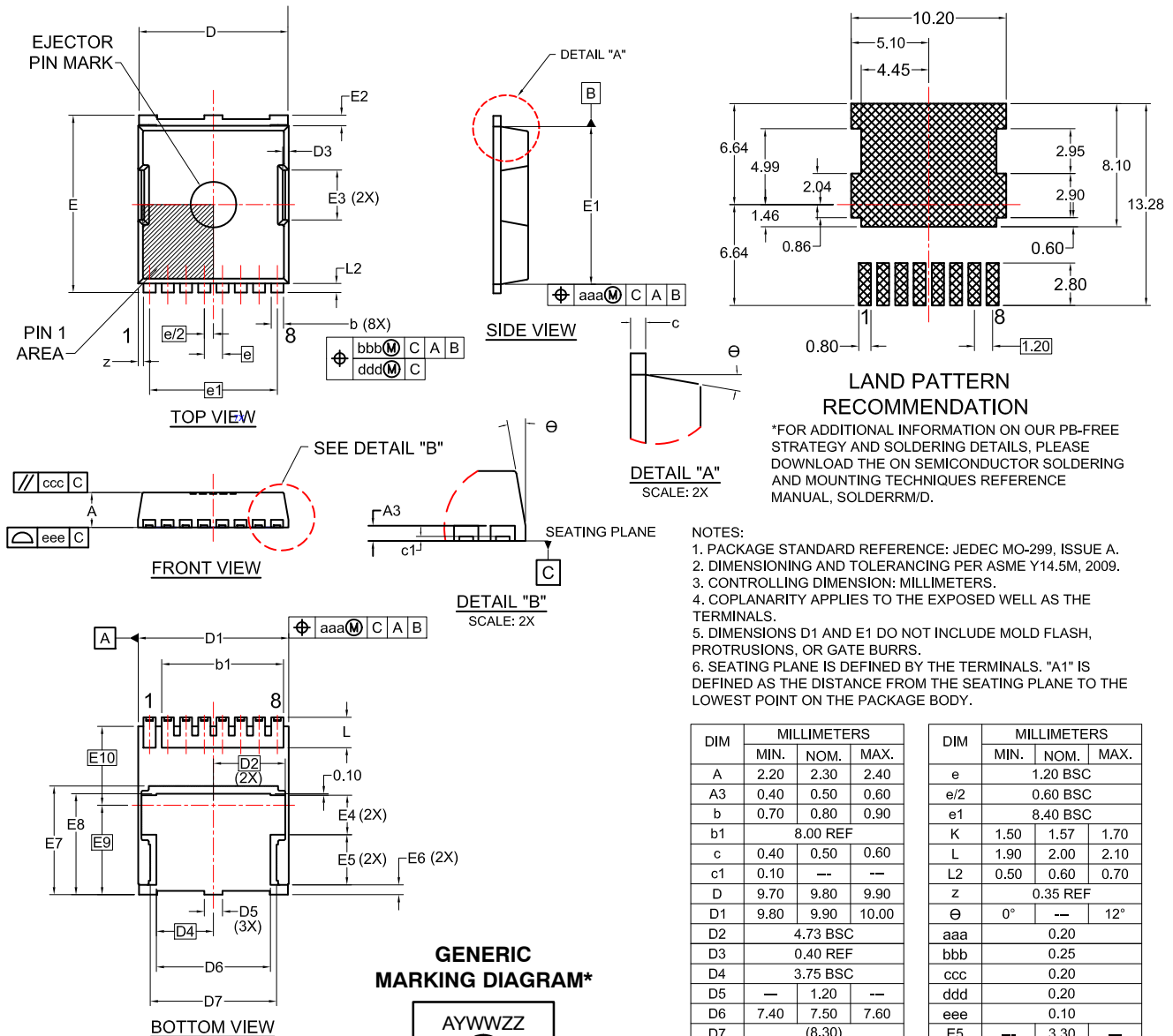
H-PSOF8L 11.68x9.80 CASE 100CU ISSUE A
