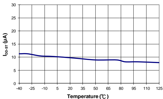
Figure 9. Startup Current
