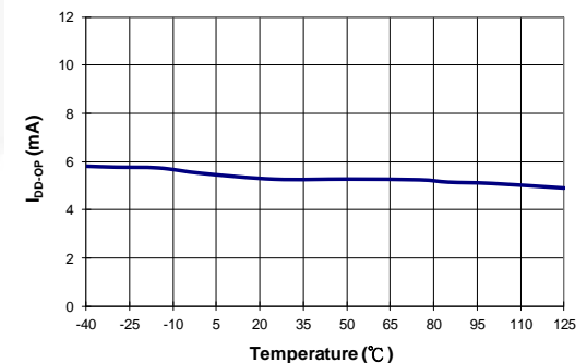
Figure 10. Operating Current
