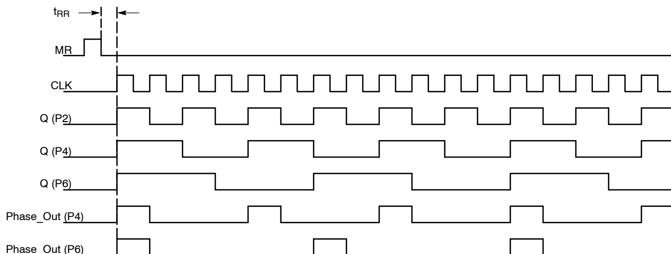
Figure 3. Timing Diagram
