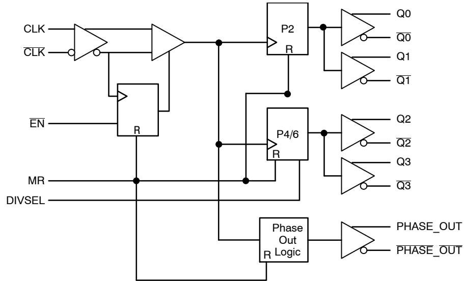
Figure 2. Logic Diagram
