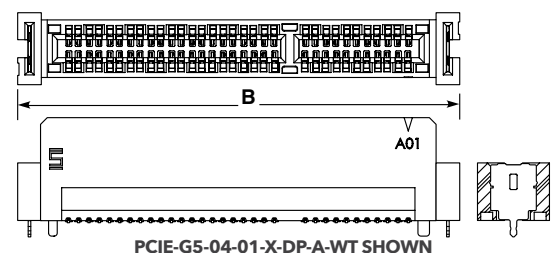
PCIE-G5-04-01-X-DP-A-WT SHOWN
