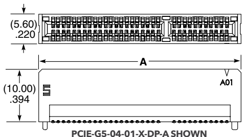
PCIE-G5-04-01-X-DP-A SHOWN
