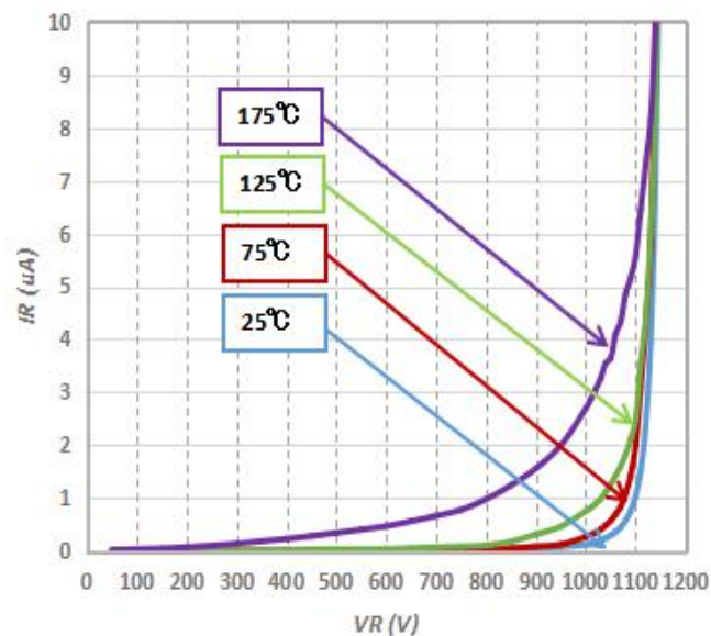
Fig.2-Typical Reverse Characteristics
