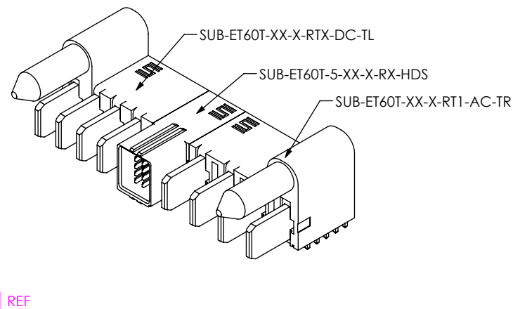
FIG 11 ET60T-D04-5-03-A04-X-RX-T SHOWN (DIFFERENT AS SHOWN, OTHERWISE SAME AS FIG 4)
