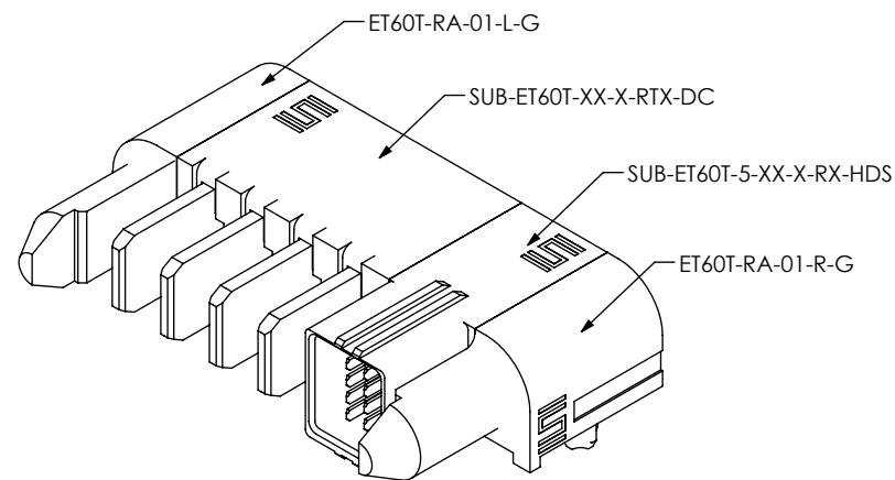
FIG 6 ET60T-D04-5-03-000-X-RX-S SHOWN (DIFFERENT AS SHOWN, OTHERWISE SAME AS FIG 4)
