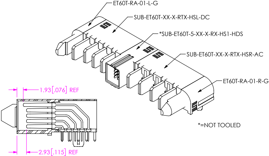
SECTION "G"-"G" FIG 13 ET60T-D04-5-03-A04-X-RX-S-H SHOWN (DIFFERENT AS SHOWN, OTHERWISE SAME AS FIG 12)
