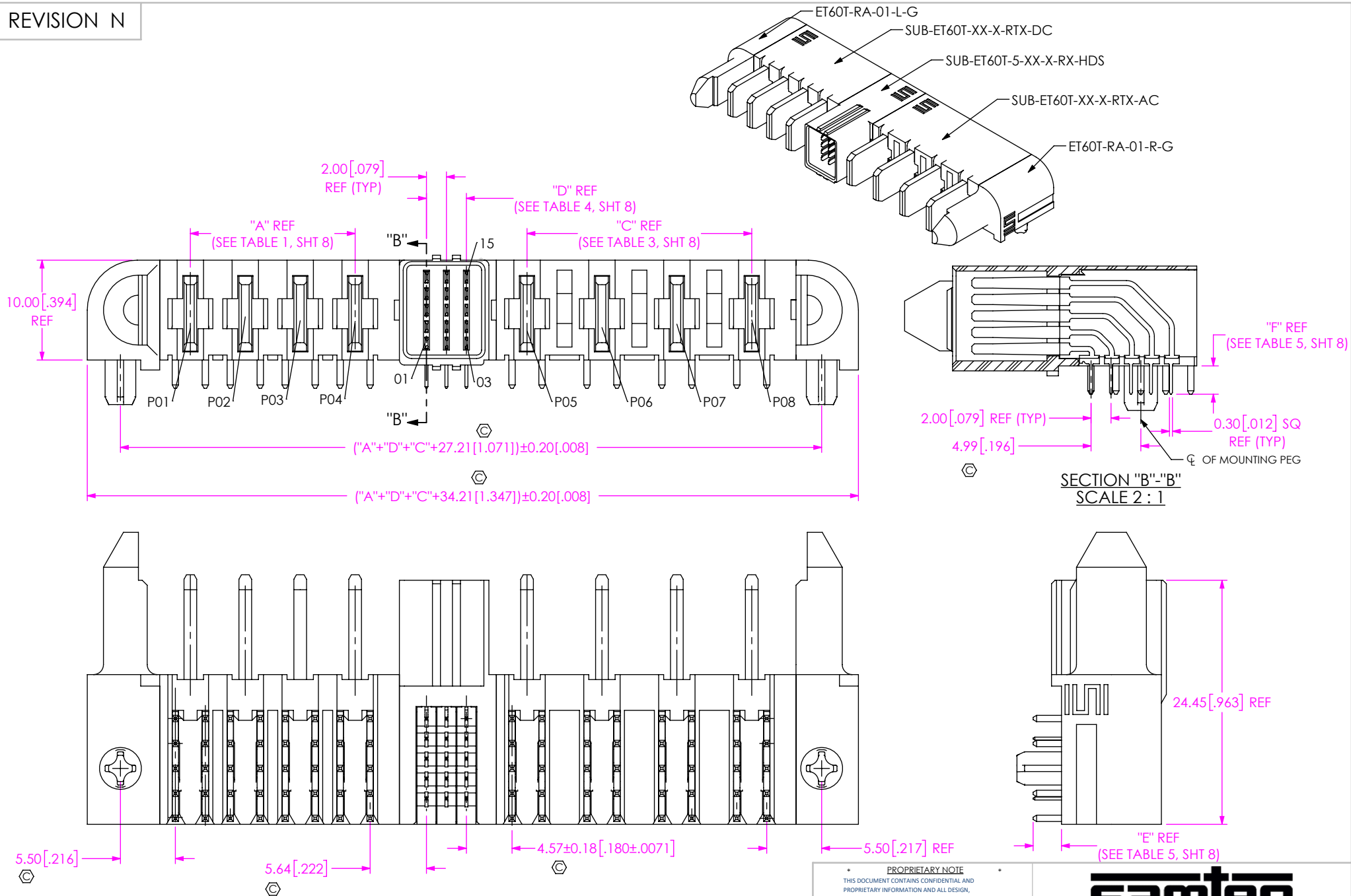
FIG 4 ET60T-D04-5-03-A04-X-RX-S SHOWN (DIFFERENT AS SHOWN, OTHERWISE SAME AS FIG 1)
