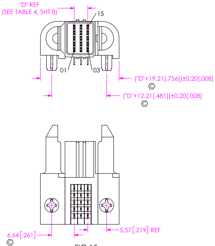
FIG 15 ET60T-000-5-03-000-X-RX-S SHOWN (DIFFERENT AS SHOWN, OTHERWISE SAME AS FIG 4)
