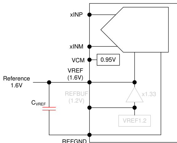
Figure 8-16. External 1.6V reference
