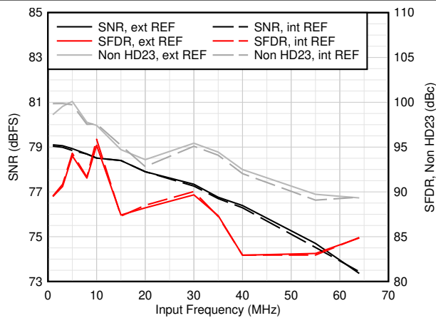
Figure 6-9. AC Performance vs Input Frequency
