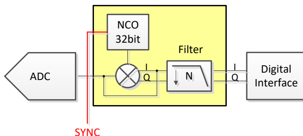
Figure 8-18. Internal Digital Decimation Filter
