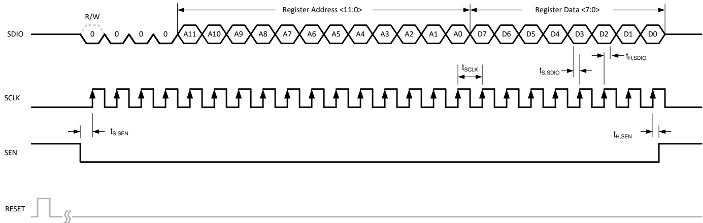
Figure 8-41. Serial Register Write Timing Diagram
