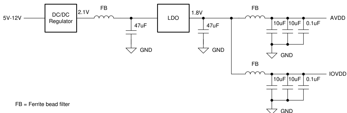
Figure 11-2. Example: LDO Linear Regulator Approach
