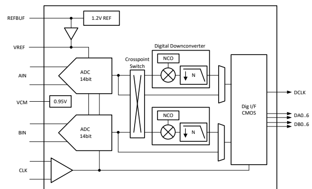
ADC364x Block Diagram
