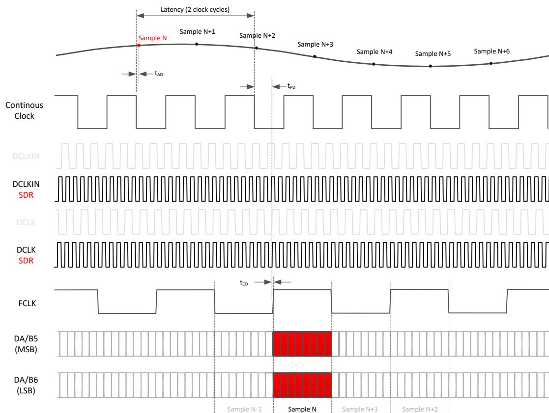
Figure 8-38. SDR Output Clocking
