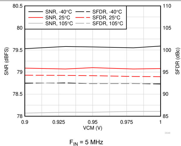
Figure 6-15. AC Performance vs VCM vs Temperature
