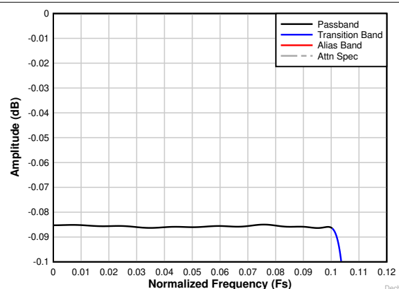
Figure 8-27. Decimation by 4 complex passband ripple response
