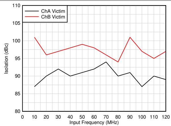
Figure 6-17. Isolation vs Input Frequency
