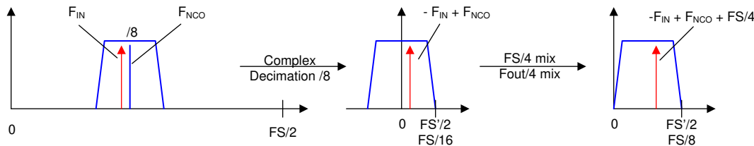
Figure 8-22. FS/4 Mixing with real output
