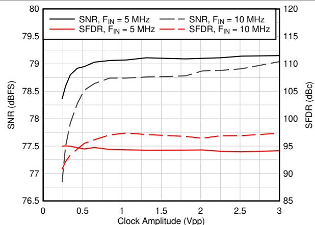
Figure 6-13. AC Performance vs Clock Amplitude
