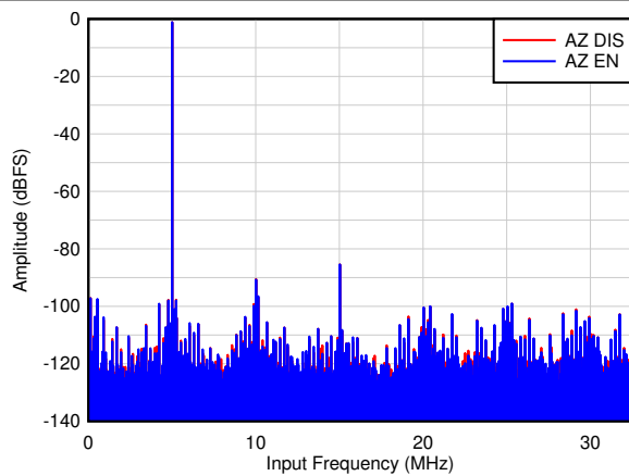
Figure 8-11. ADC3643: FFT at 65 MSPS with input frequency of 5 MHz (auto-zero feature enable vs disable, 4M point FFT)
