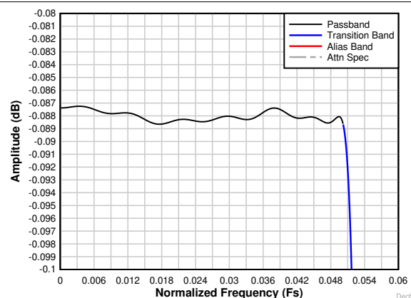
Figure 8-29. Decimation by 8 complex passband ripple response
