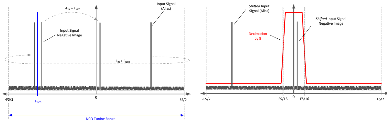
Figure 8-20. Complex decimation illustration
