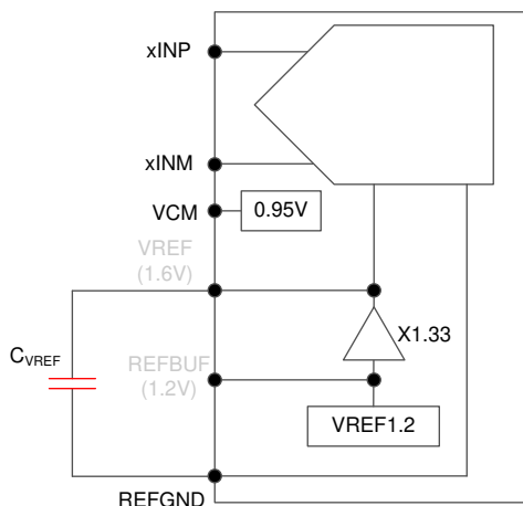
Figure 8-15. Internal reference
