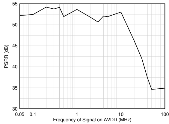
Figure 11-1. Power supply rejection ratio (PSRR) vs frequency
