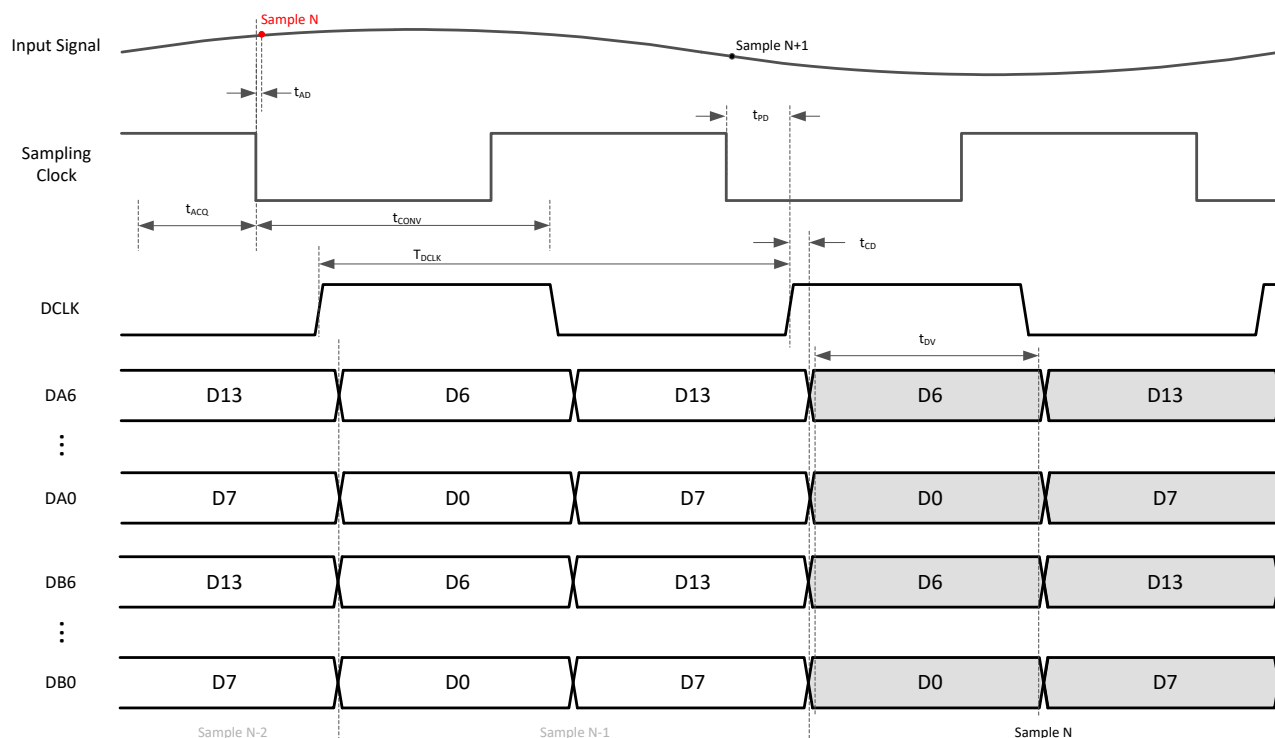
Figure 7-1. Timing diagram: DDR CMOS
