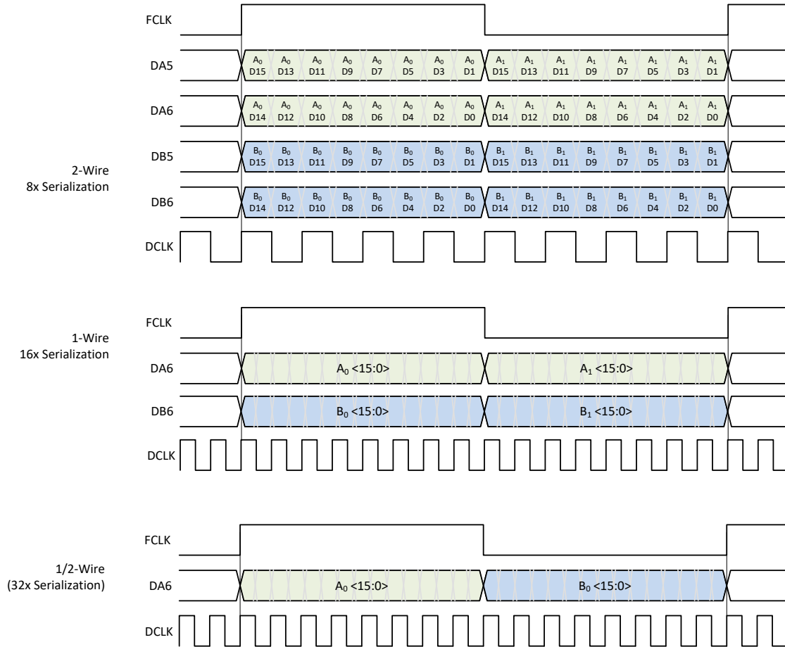
Figure 8-37. Output Data Format in Real Decimation
