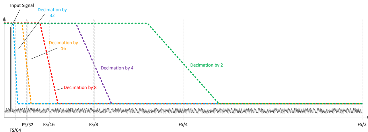
Figure 8-21. Real decimation illustration
