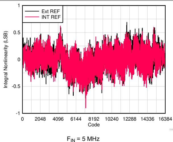
Figure 6-18. INL vs Code
