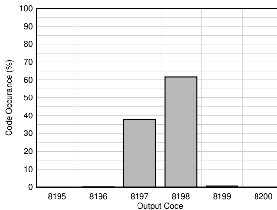
Figure 6-20. DC Histogram
