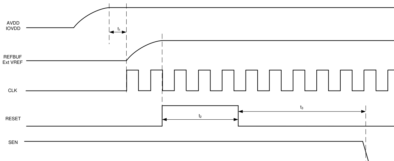
Figure 10-1. Initialization of serial registers after power up
