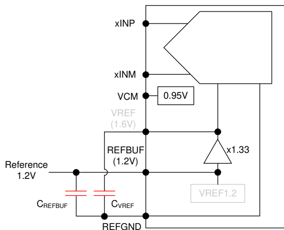
Figure 8-17. External 1.2V reference using internal reference buffer
