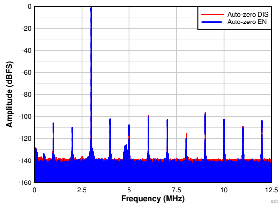
Figure 8-9. FFT at 25 MSPS with input frequency of 3 MHz (auto-zero feature enable vs disable, 4M point FFT)
