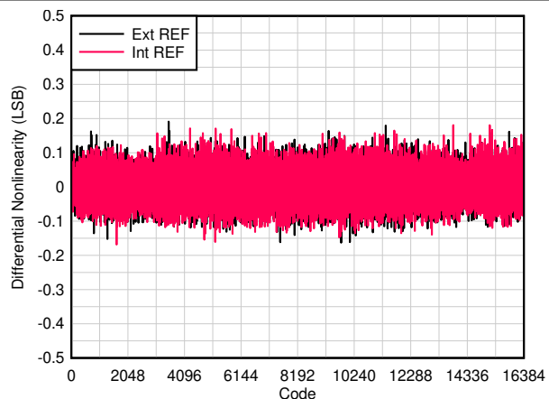
Figure 6-19. DNL vs Code
