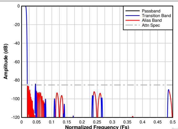
Figure 8-32. Decimation by 32 complex frequency response
