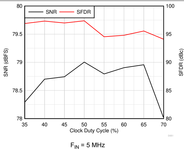
Figure 6-16. AC Performance vs Clock Duty Cycle
