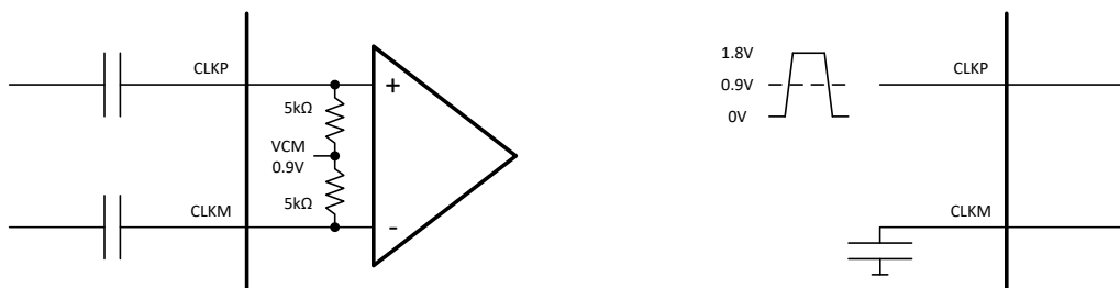
Figure 8-13. External and internal connection using differential (left) and single ended (right) clock input
