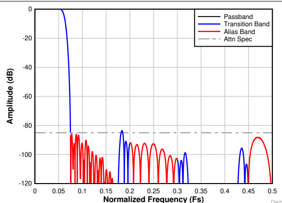
Figure 8-28. Decimation by 8 complex frequency response
