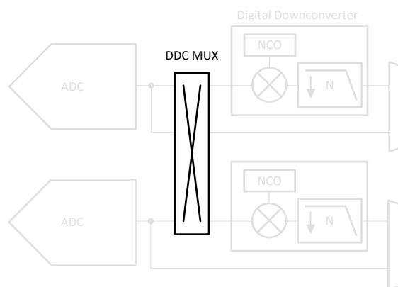
Figure 8-19. DDC MUX
