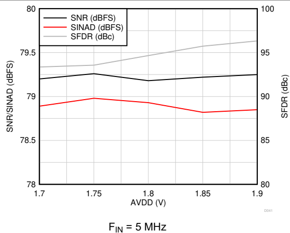
Figure 6-14. AC Performance vs AVDD
