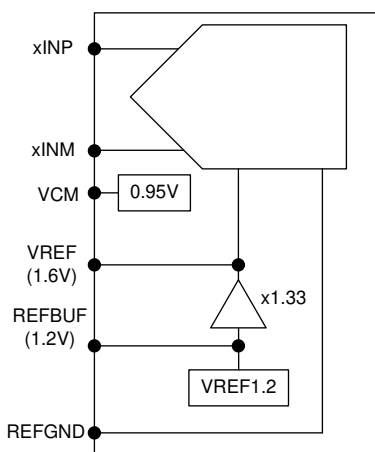
Figure 8-14. Different voltage reference options for ADC364x
