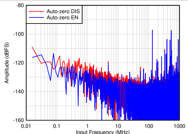
Figure 8-12. ADC3643: FFT at 65 MSPS with input frequency of 5 MHz (auto-zero feature enabled vs disabled, 4M point FFT)
