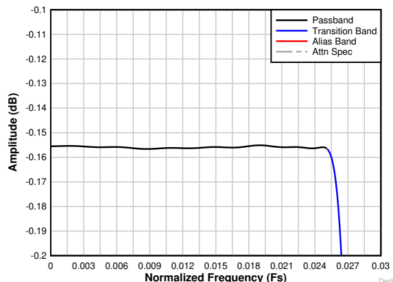
Figure 8-31. Decimation by 16 complex passband ripple response
