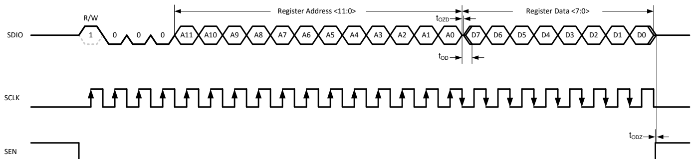
Figure 8-42. Serial Register Read Timing Diagram
