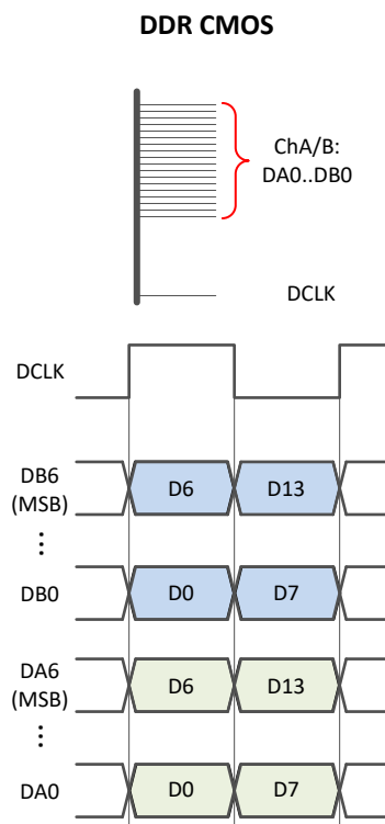
Figure 8-35. Output Data Format in Real Decimation
