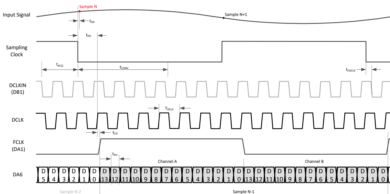
Figure 7-4. Timing diagram: 1/2-wire serial CMOS
