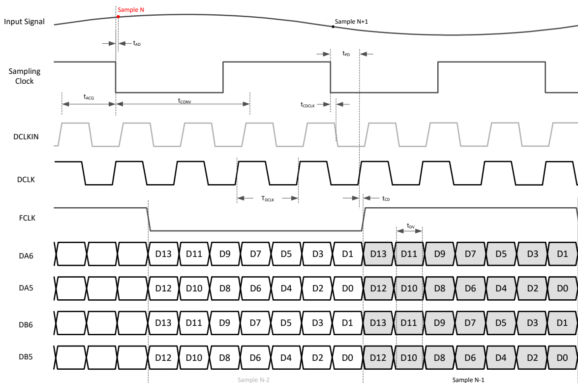
Figure 7-2. Timing diagram: 2-wire serial CMOS
