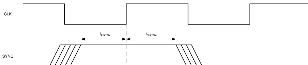
Figure 8-34. External SYNC timing diagram
