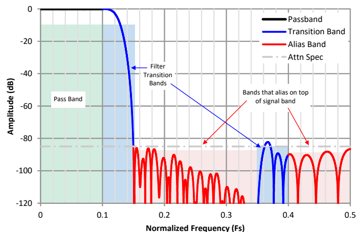
Figure 8-23. Interpretation of the Decimation Filter Plots
