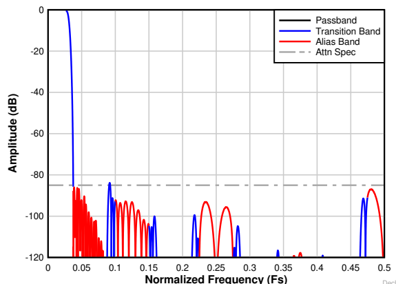
Figure 8-30. Decimation by 16 complex frequency response
