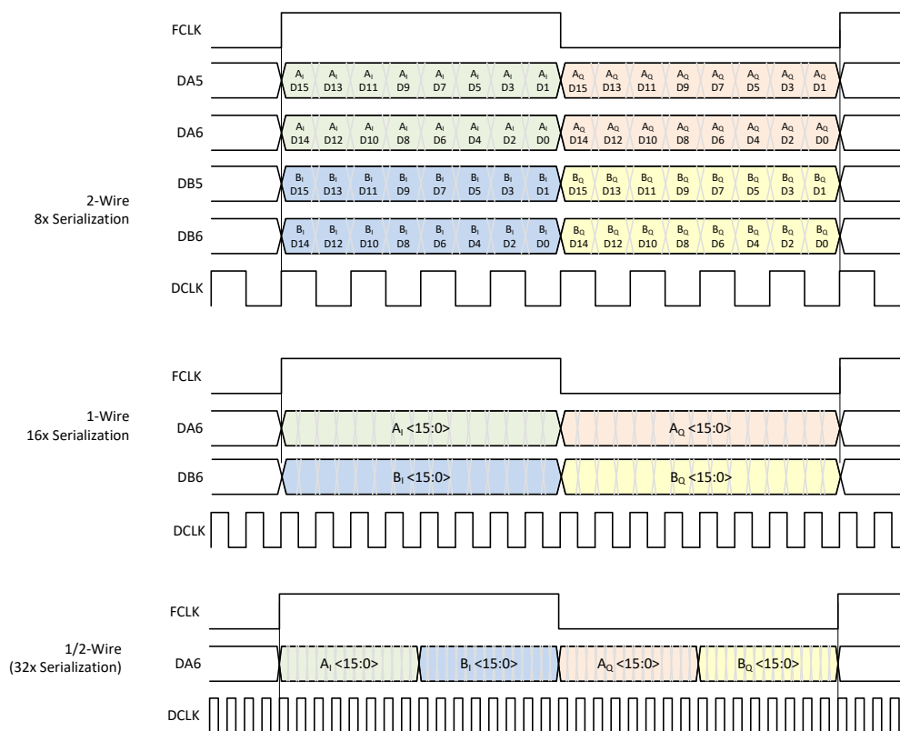
Figure 8-36. Output Data Format in Complex Decimation
