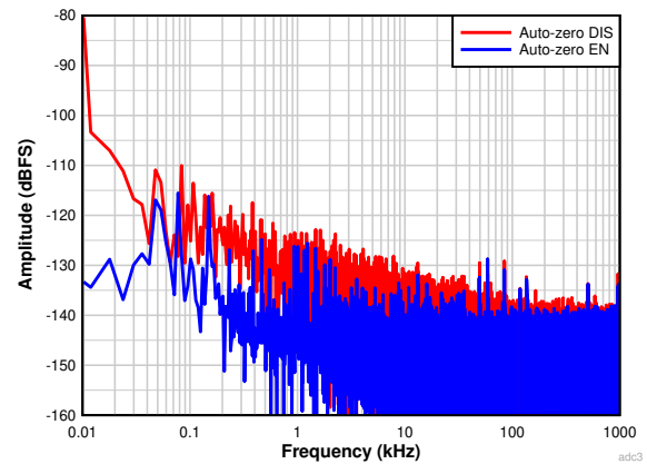
Figure 8-10. FFT at 25 MSPS with input frequency of 3 MHz (auto-zero feature enable vs disable, 4M point FFT)
