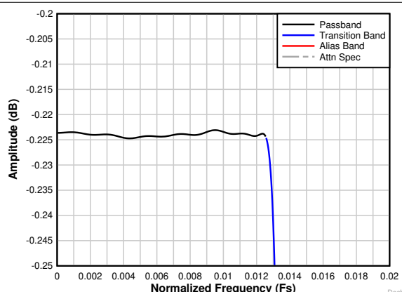
Figure 8-33. Decimation by 32 complex passband ripple response
