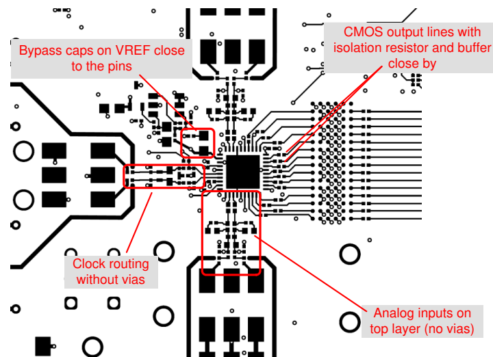
Figure 12-1. Layout example: top layer of ADC364x EVM
