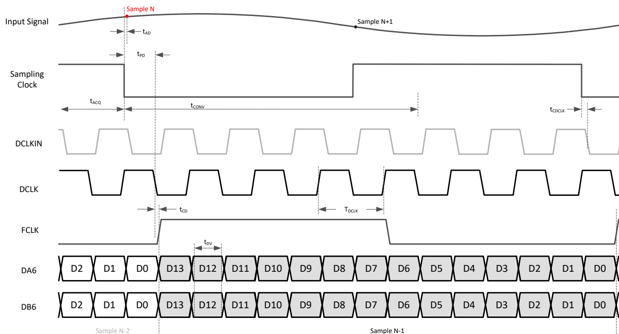
Figure 7-3. Timing diagram: 1-wire serial CMOS
