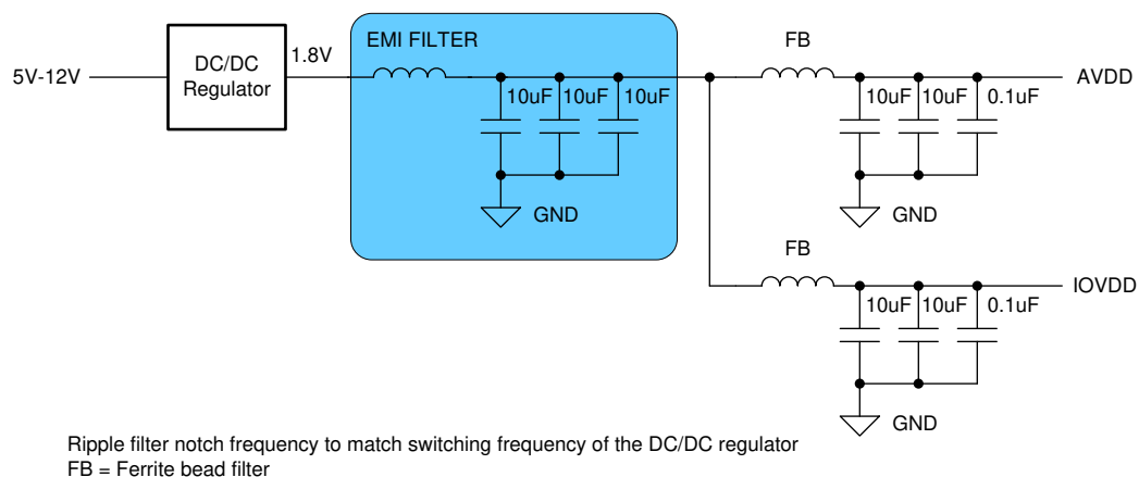
Figure 11-3. Example Switcher-Only Approach
