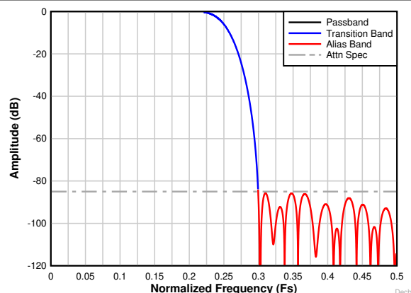
Figure 8-24. Decimation by 2 complex frequency response
