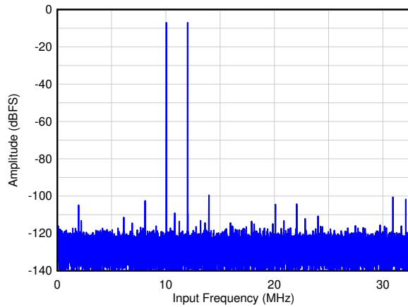
Figure 6-7. Two Tone FFT at F_{IN} = 10/12 MHz
