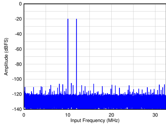
Figure 6-8. Two Tone FFT at F_{IN} = 10/12 MHz
