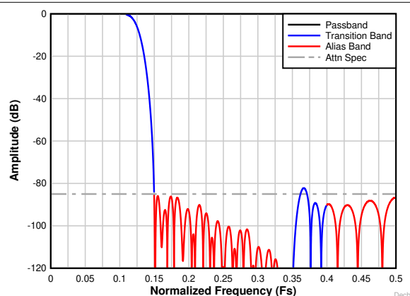
Figure 8-26. Decimation by 4 complex frequency response
