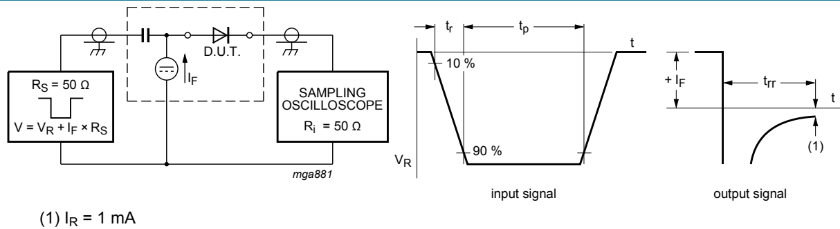
Fig. 15. Reverse recovery time: test circuit and waveforms
