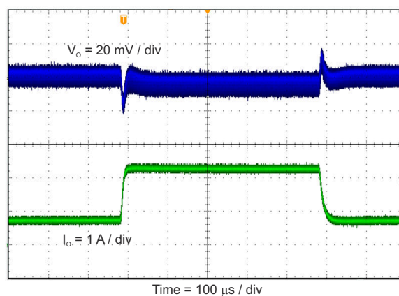
Figure 4-5. Load Transient Response, 25% to 75% Load Step
