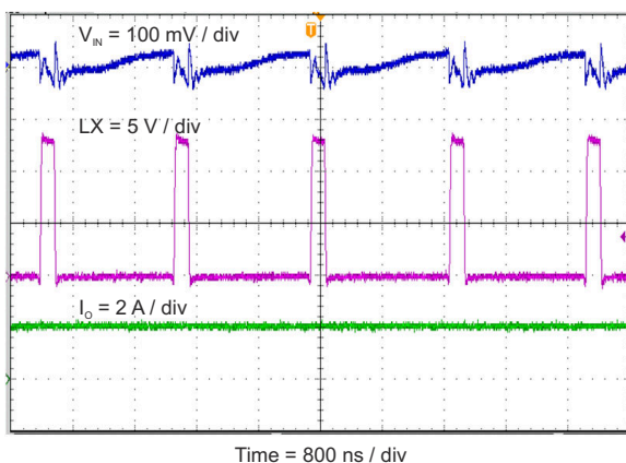
Figure 4-9. Input Voltage Ripple, I_{OUT} = 3\text{ A}
