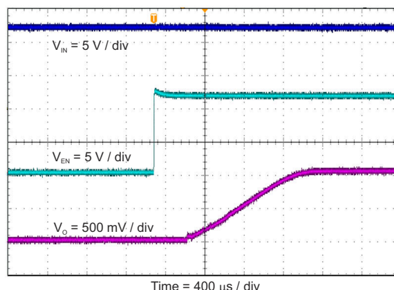
Figure 4-11. Start-Up Relative to EN
