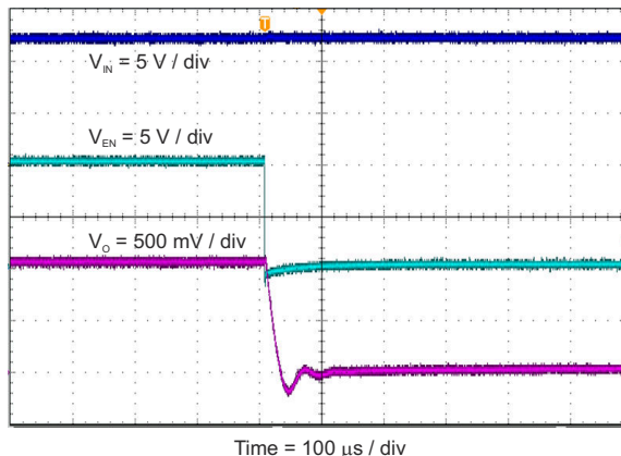
Figure 4-13. Shut-Down Relative to EN
