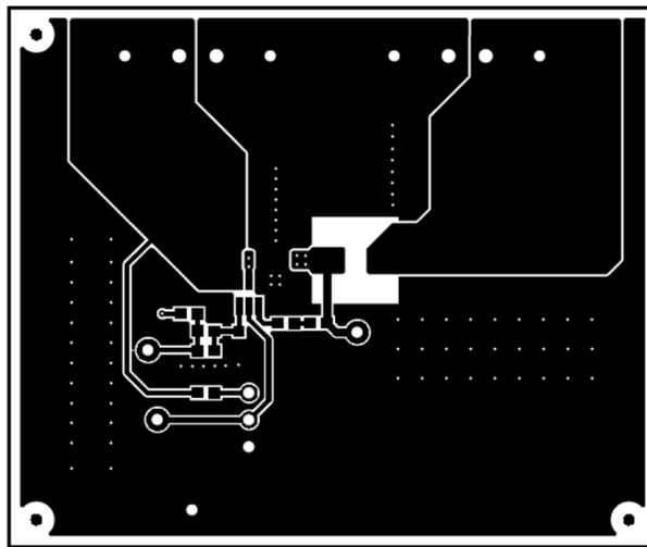
Figure 5-2. Top Layer
