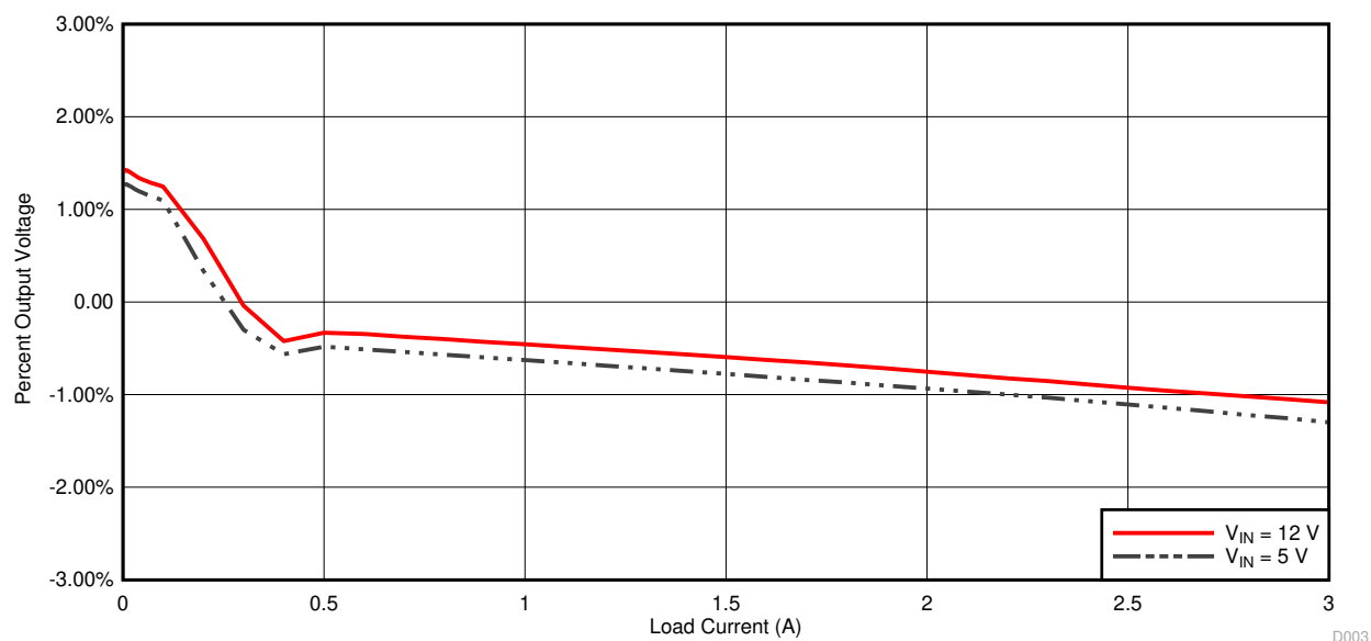
Figure 4-3. Load Regulation
