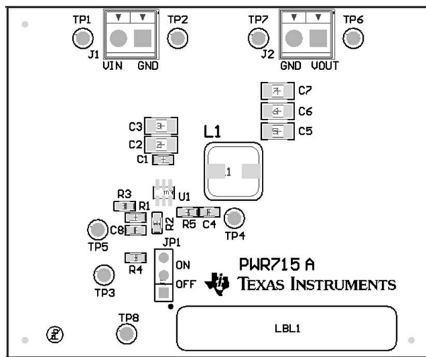
Figure 5-1. Top Assembly
