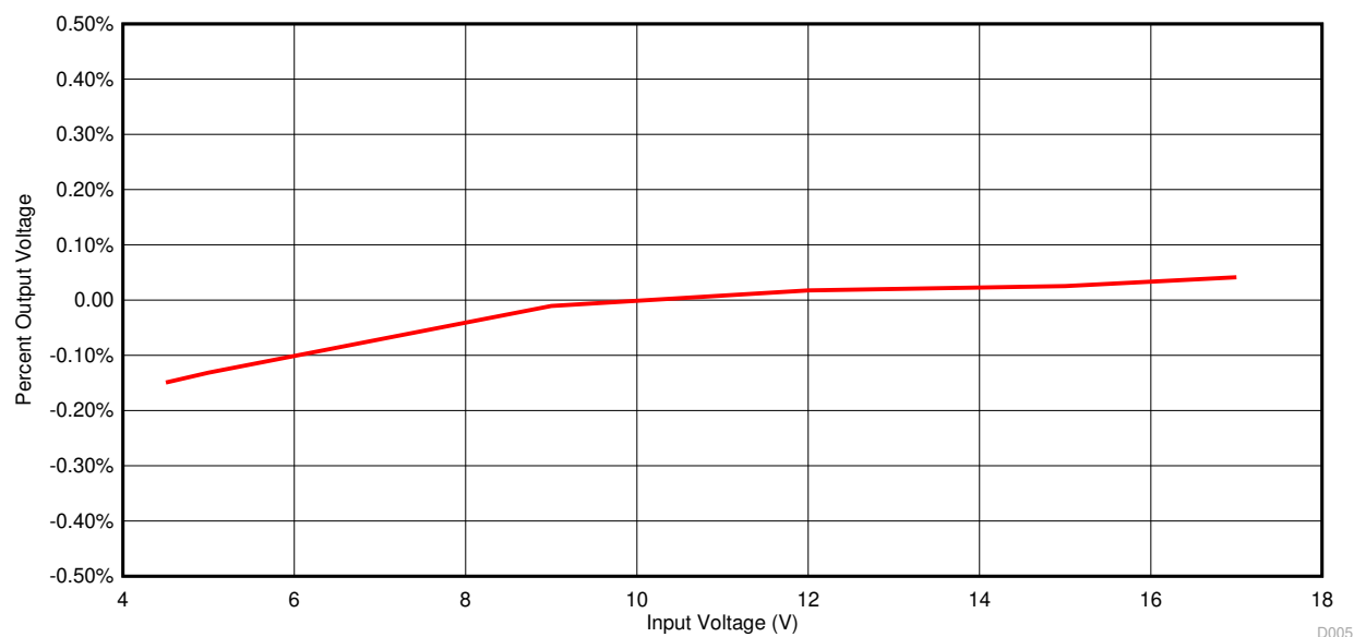
Figure 4-4. Line Regulation
