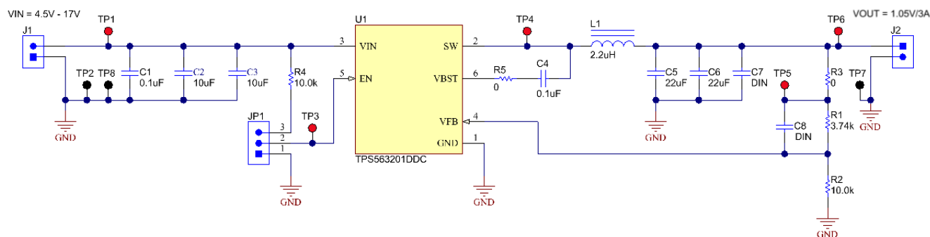
Figure 6-1. TPS563201EVM-715 Schematic Diagram
