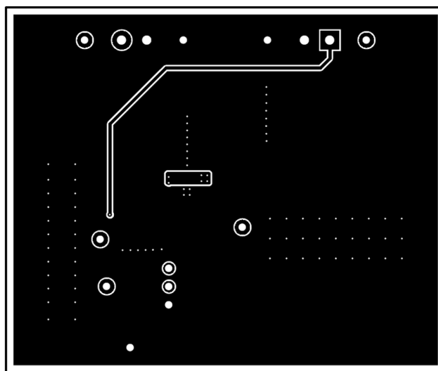
Figure 5-3. Bottom Layer
