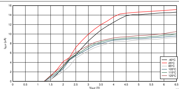
Figure 10-9. I_{SUP} vs V_{SUP} vs Temperature Ramp-down
