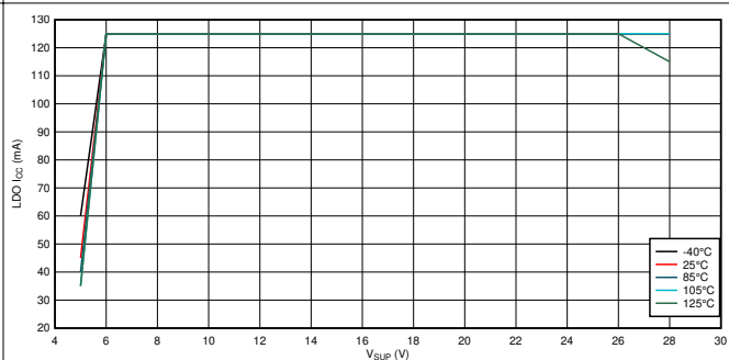
Figure 7-4. I_{CC} vs V_{SUP} vs Temperature
