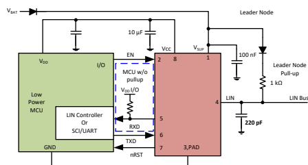
Simplified Schematics, Leader Node (1)
