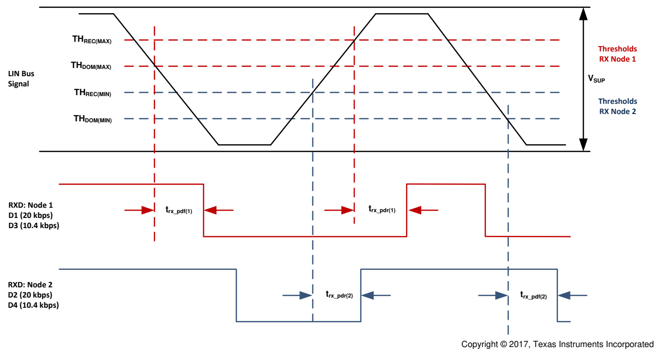
Figure 8-14. Propagation Delay
