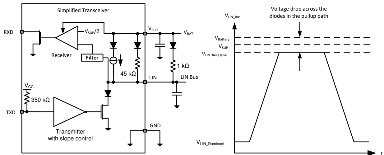
Figure 9-2. Leader Node Configuration with Voltage Levels
