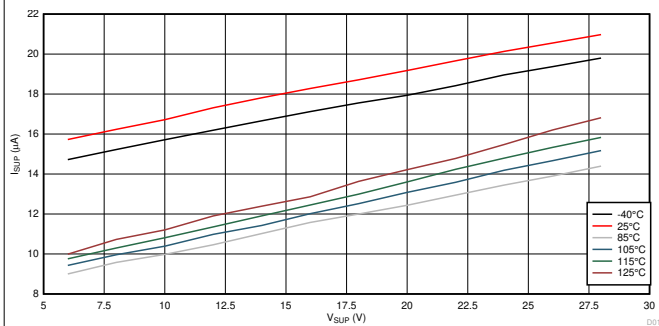
Package = DRB V_{CC} = 5\text{ V} Temp = Ambient
