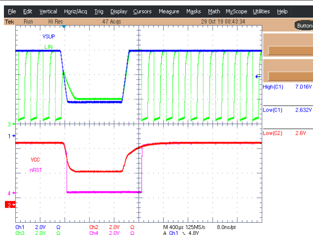
Figure 10-18. TLIN10285-Q1 Brownout
