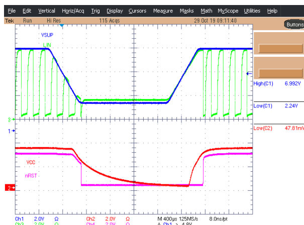
Figure 10-17. TLIN10283-Q1 Brownout
