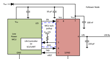
Simplified Schematics, Follower Node (2)
