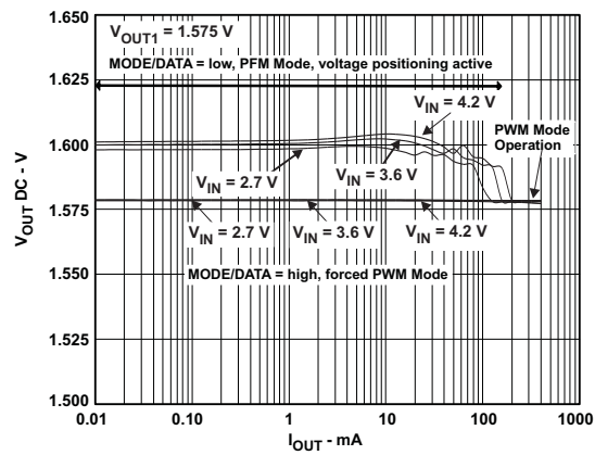
Figure 28. DC Output Accuracy VOUT1 = 1.575V, L = 2.2μH, COUT = 22μF
