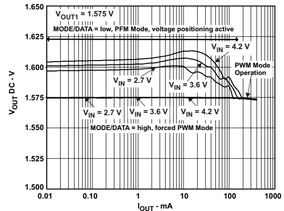
Figure 29. DC Output Accuracy VOUT1 = 1.575V, L = 3.3μH, COUT = 10μF
