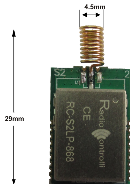
915MHz version with Helical Antenna
