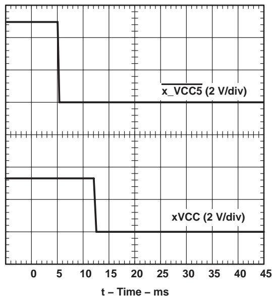
Figure 7. xVCC Propagation Delay and Fall Time With 1-μF Load, 3.3-V Switch, V_{I(5V)} = 0
