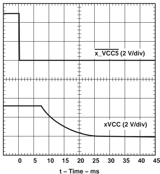
Figure 9. xVCC Propagation Delay and Fall Time With 150-μF Load, 3.3-V Switch, V_{I(5V)} = 0
