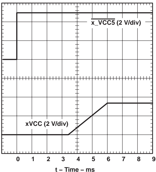
Figure 6. xVCC Propagation Delay and Rise Time With 1-μF Load, 3.3-V Switch, V_{I(5V)} = 0
