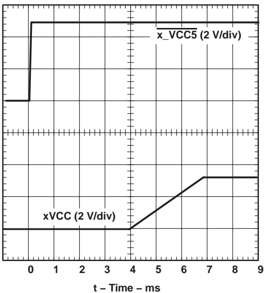
Figure 8. xVCC Propagation Delay and Rise Time With 150-μF Load, 3.3-V Switch, V_{I(5V)} = 0
