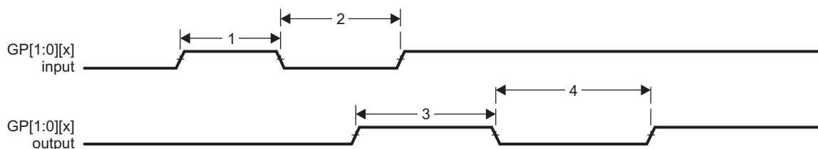
Figure 9-49. GPIO Port Timing
