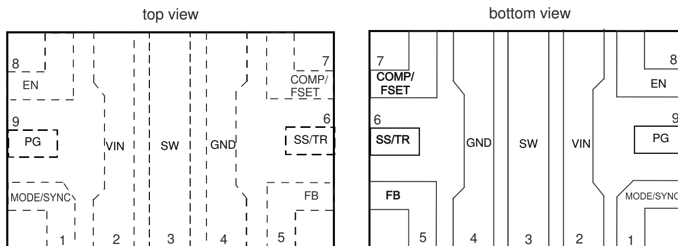
Figure 6-1. RWY Package 9 Pin (VQFN) Top View
