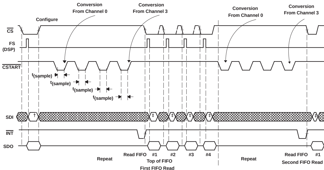
Figure 13. TLV1504/TLV1508 Mode 10/11 DSP Serial Interface (Conversions Triggered by \overline{\text{CSTART}} )
