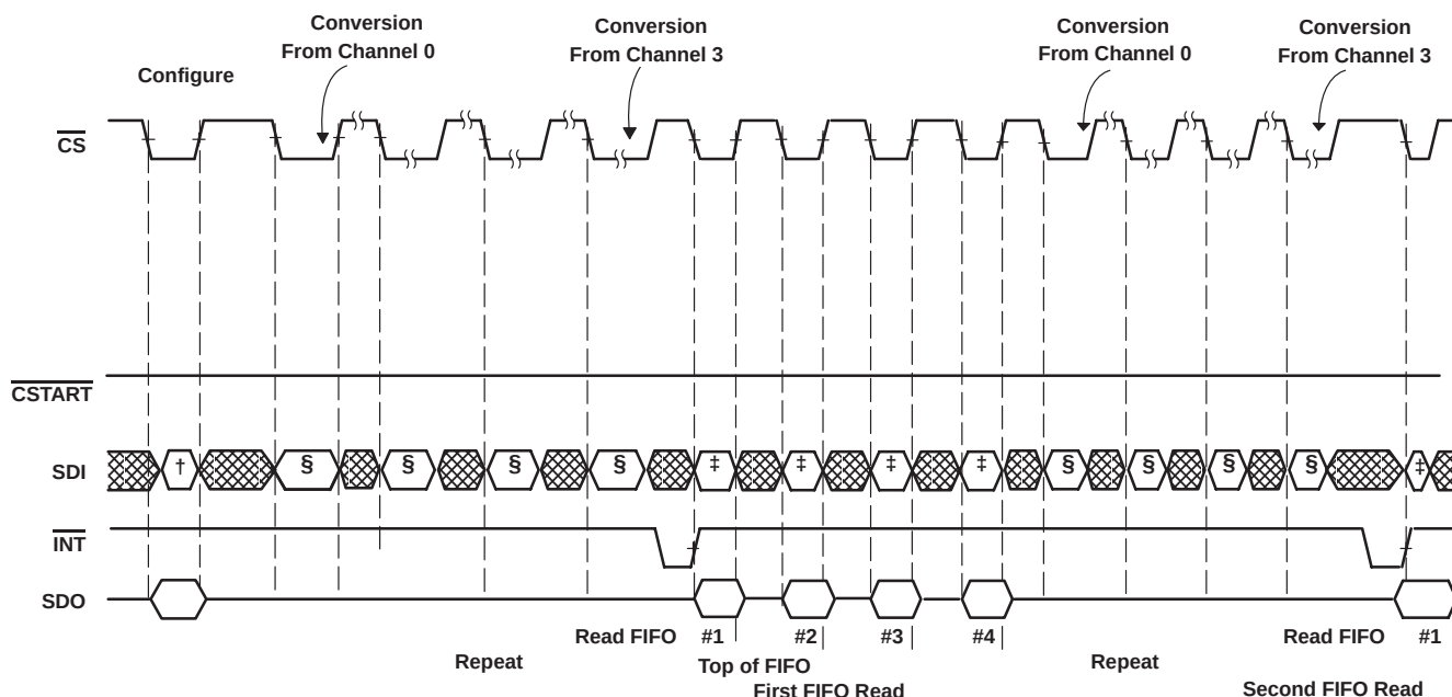
Figure 13. TLV1504/TLV1508 Mode 10/11 DSP Serial Interface (Conversions Triggered by \overline{\text{CSTART}} )
