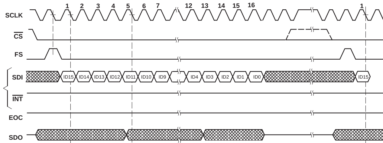
Figure 5. TLV1504/TLV1508 Write Cycle (FS Active)
