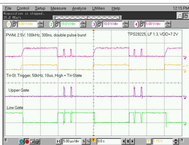
Figure 22. 2.5-V Amplitude PWM Pulse (TPS28225 example)
