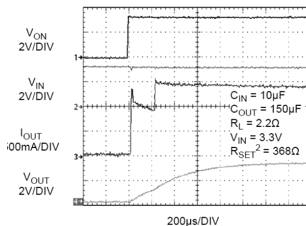
Figure 24. Short-Circuit Detection Function (4)
