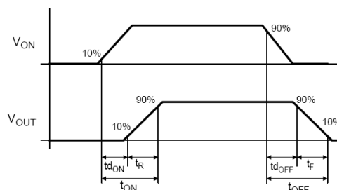
Figure 27. Timing Diagram
