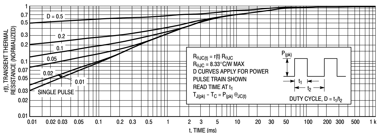
Figure 6. Thermal Response
