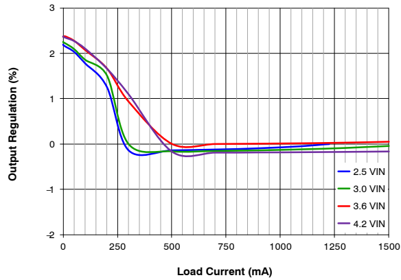
Figure 11. Output Regulation vs. Load Current and Input Voltage (Normalized to 3.6\text{ V}_{IN} , 500 mA Load)
