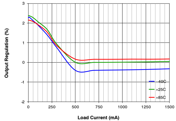
Figure 12. Output Regulation vs. Load Current and Temperature (Normalized to 3.6\text{ V}_{IN} , 500 mA Load, T_A = 25^\circ\text{C} )
