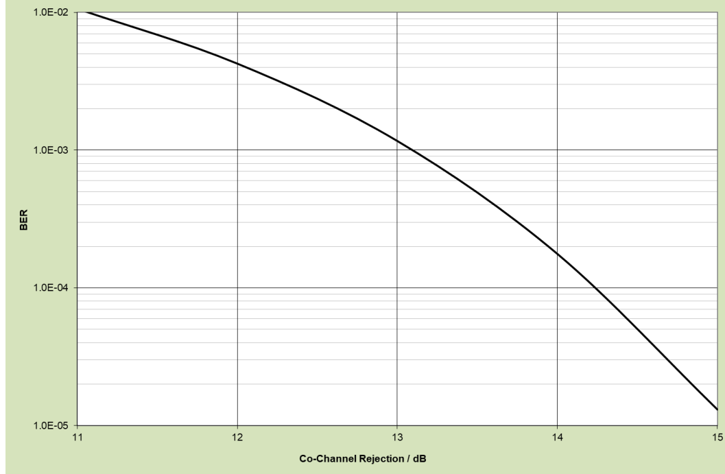
Figure 77 Co-Channel Rejection Performance at 20ksymbols/s – Uncoded (raw) 4-FSK
