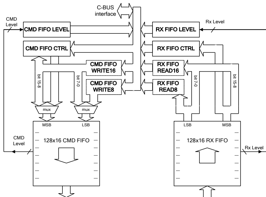
Figure 35 Command and Rx Data FIFOs
