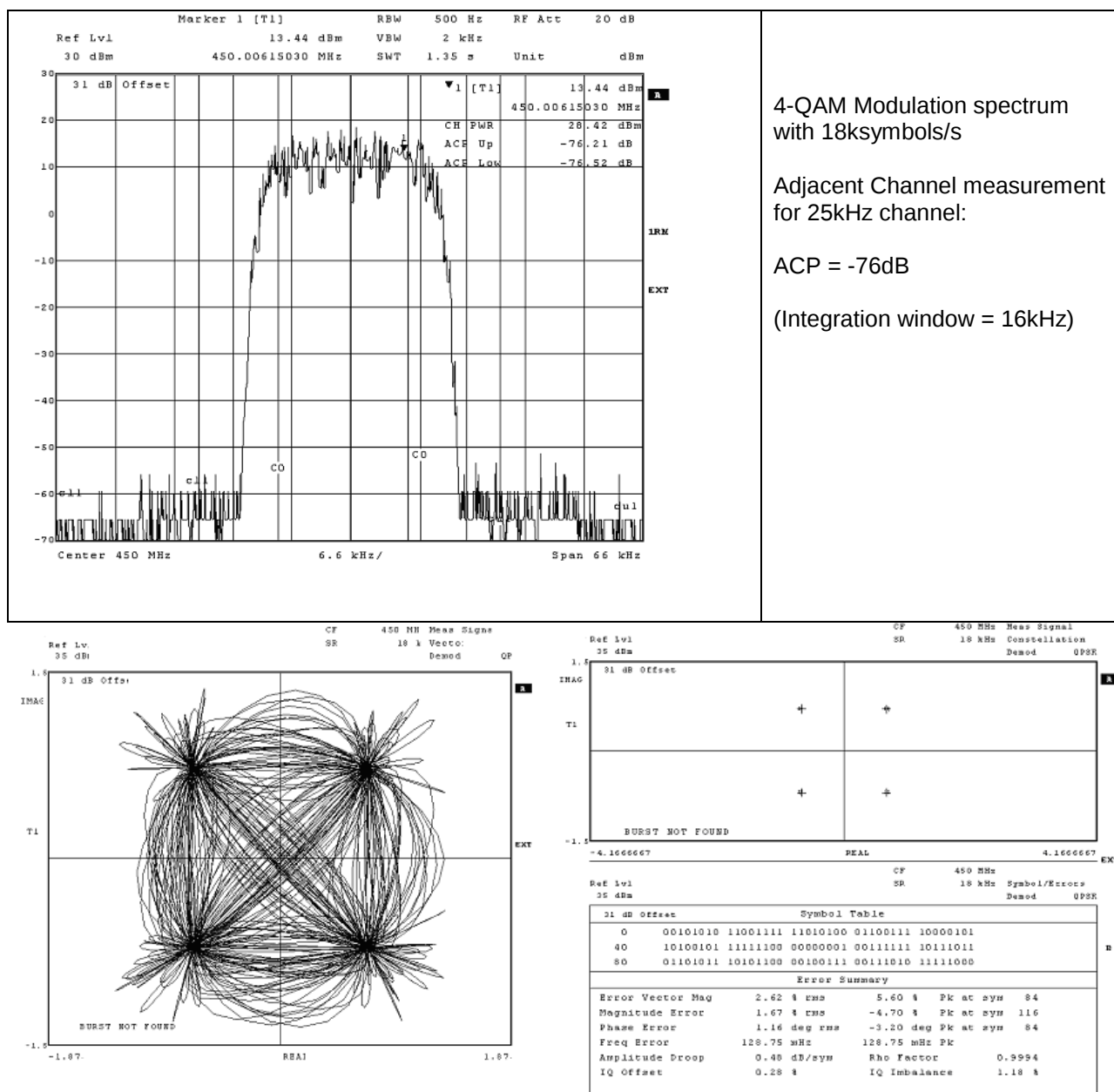
Constellation Diagram (Receiver filtered)
