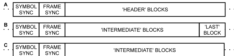
Figure 56 Suggested Frame Structures
