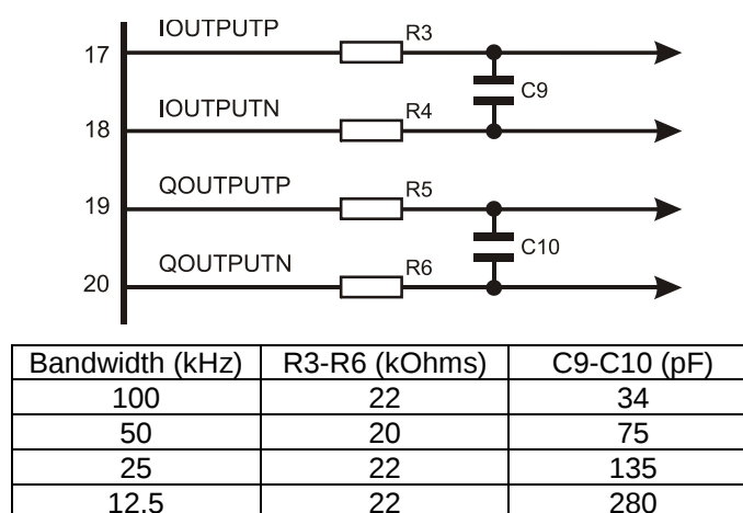
Figure 8 Recommended External Components – I/Q Output Reconstruction Filter
