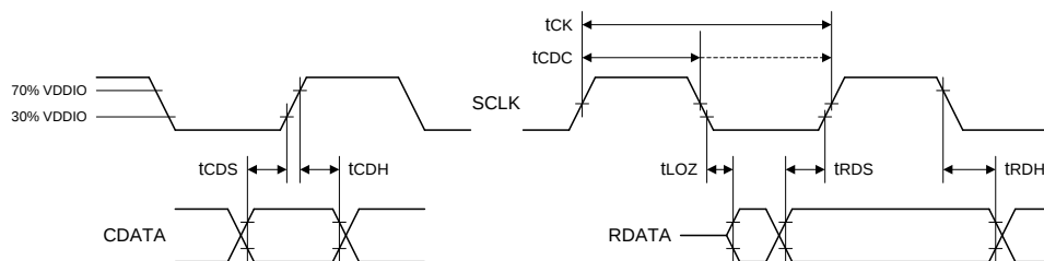
Figure 114 C-BUS Timing
