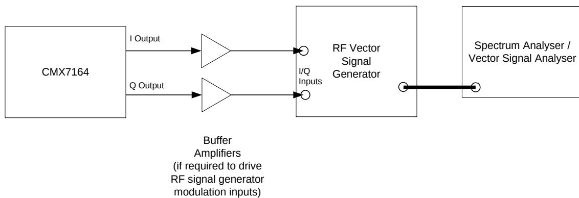
Figure 44 Tx Spectrum and Modulation Measurement Configuration for I/Q Operation
