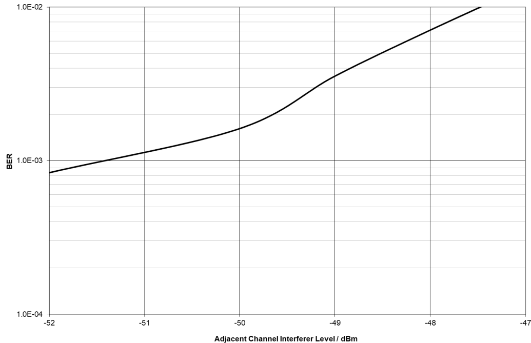
Figure 78 ACR Performance
