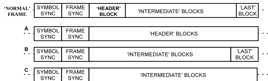
Figure 85 Suggested Frame Structures
