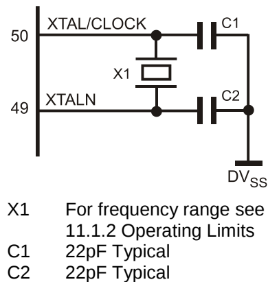
Figure 6 Recommended External Components – Xtal Interface
