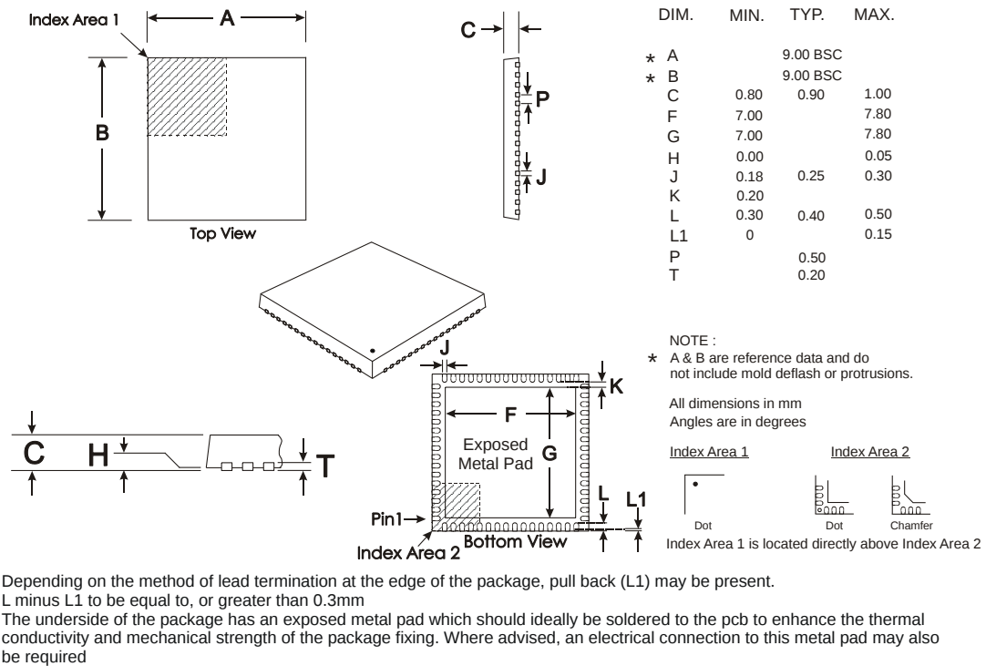
Figure 115 Mechanical Outline of 64-pin VQFN (Q1)
