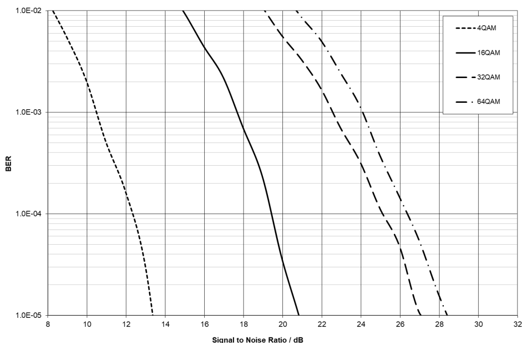
Figure 94 Modem Sensitivity Performance at 18ks/s
