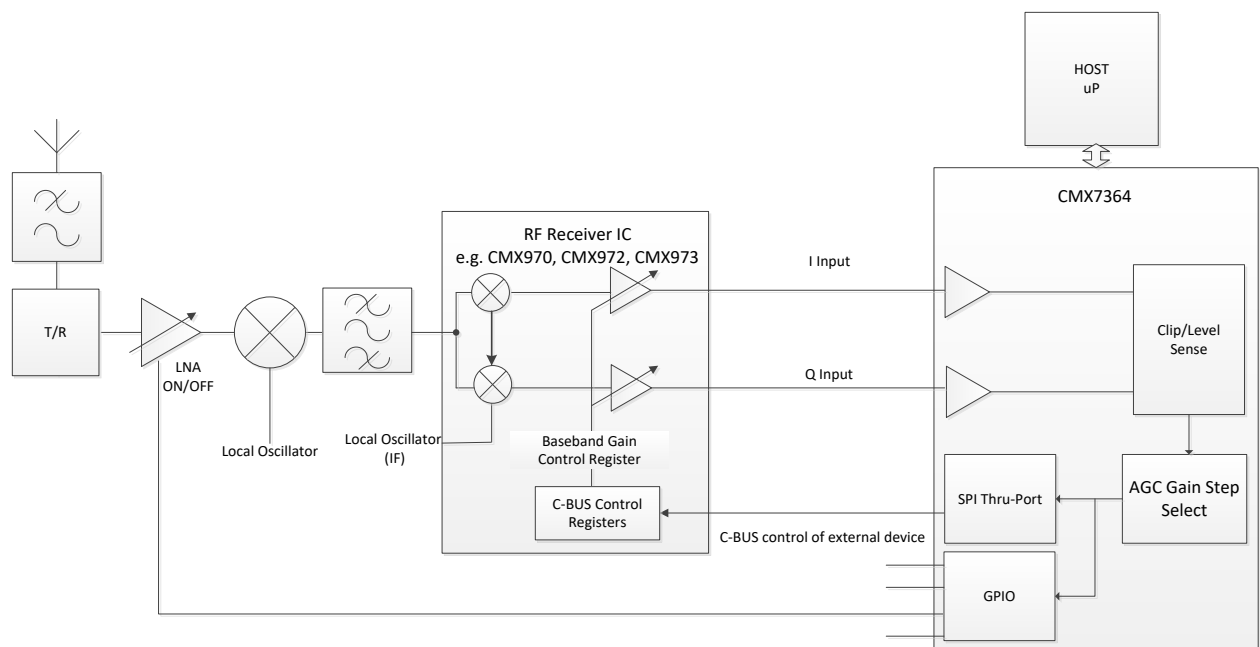
Figure 37 AGC using SPI Thru-Port and external LNA
