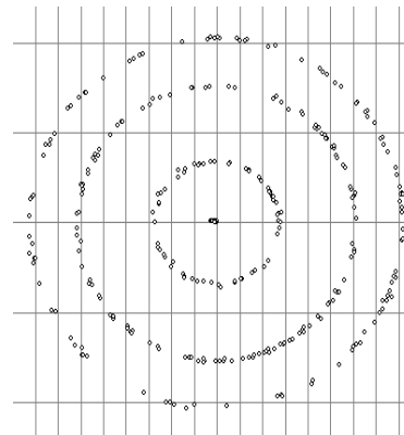
Figure 30 Sample at Symbol Timing with I/Q DC Offset Diagnostic Mode (with frequency error)
