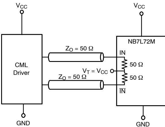
Figure 15. Standard 50 Ω Load CML Interface
