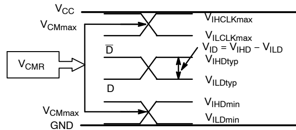
Figure 17. V_{CMR} Diagram
