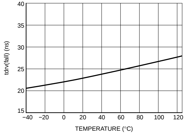
Figure 23. t_{DRV(fall)} vs. Junction Temperature
