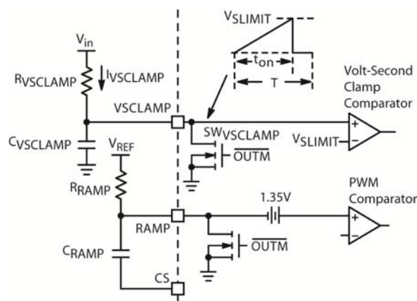
Figure 54. The VSCLAMP Configuration in Peak Current-mode Control
