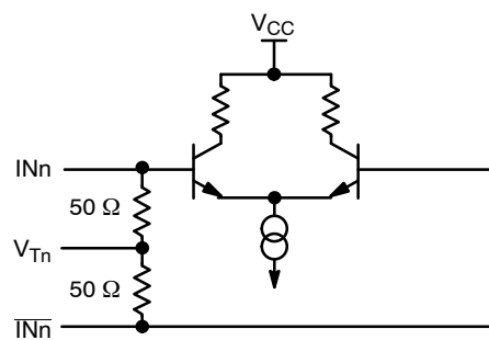
Figure 4. Input Structure
