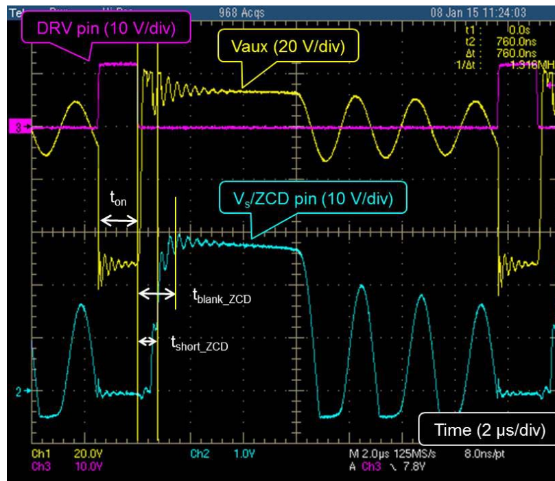
Figure 49. V_s/ZCD Pin Waveforms
