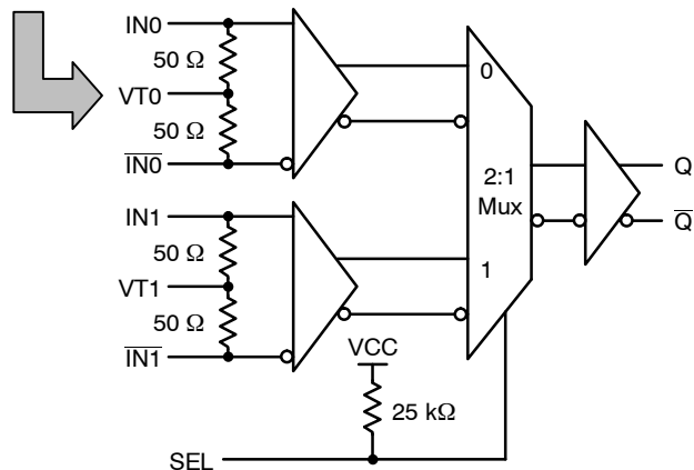
Figure 2. Detailed Block Diagram
