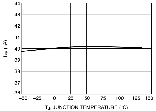
Figure 37. Line Feedforward Current on CS Pin (@ V FS = 2 V) vs. Temperature
