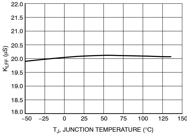
Figure 36. Feedforward V FS to I CS(offset) Conversion Ratio vs. Temperature
