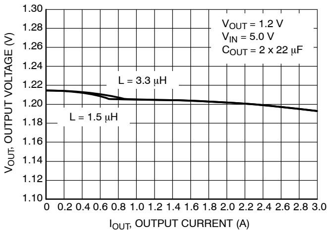
Figure 13. Load Regulation for V OUT = 1.2 V
