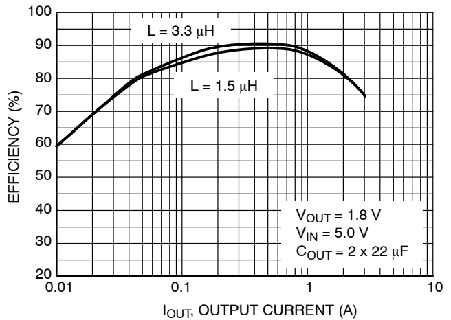
Figure 12. Efficiency vs. Output Current for V OUT = 1.8 V
