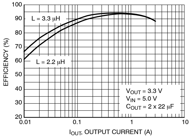
Figure 10. Efficiency vs. Output Current for V OUT = 3.3 V
