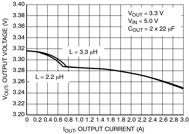
Figure 9. Load Regulation for V OUT = 3.3 V
