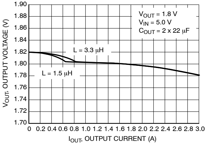
Figure 11. Load Regulation for V OUT = 1.8 V
