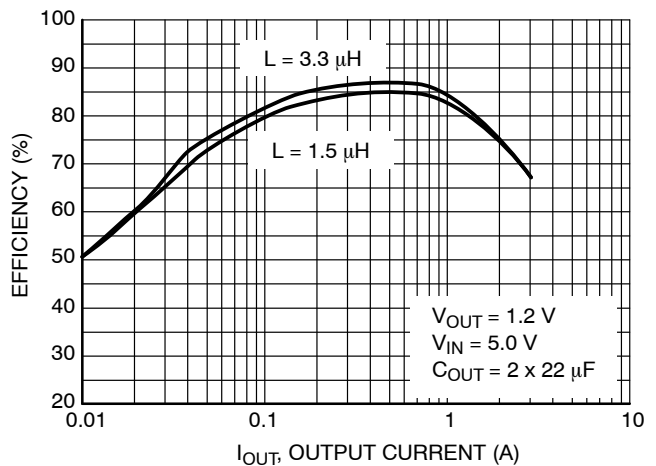
Figure 14. Efficiency vs. Output Current for V OUT = 1.2 V
