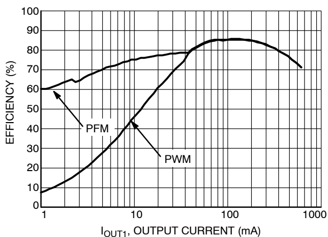
Figure 5. Efficiency vs. Output Current V_{IN} = 3.6\text{ V} , V_{OUT1} = 1.2\text{ V} , EN2 = \text{GND}
