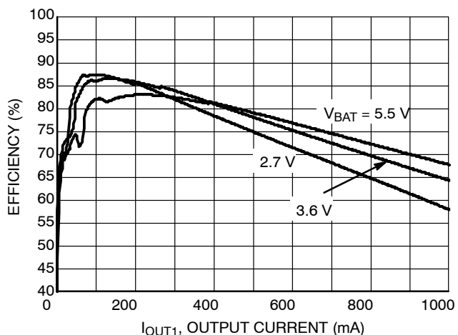
Figure 7. Efficiency vs. Output Current V_{OUT1} = 1.2\text{ V} , EN2 = \text{GND} , Temperature = 25°C
