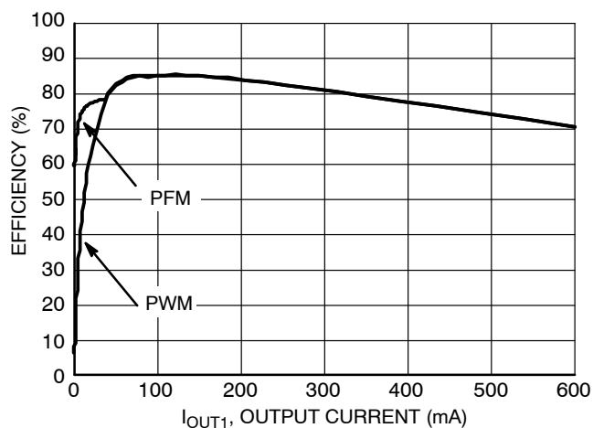
Figure 4. Efficiency vs. Output Current V_{IN} = 3.6\text{ V} , V_{OUT1} = 1.2\text{ V} , EN2 = \text{GND}
