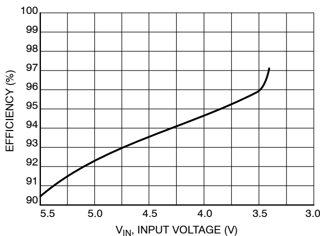
Figure 9. Maximum Efficiency vs. Input Voltage V_{OUT1} = V_{OUT2} = 3.3\text{ V} , I_{OUT1} = I_{OUT2} = 100\text{ mA}
