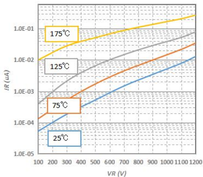
Fig.2-Typical Reverse Characteristics
